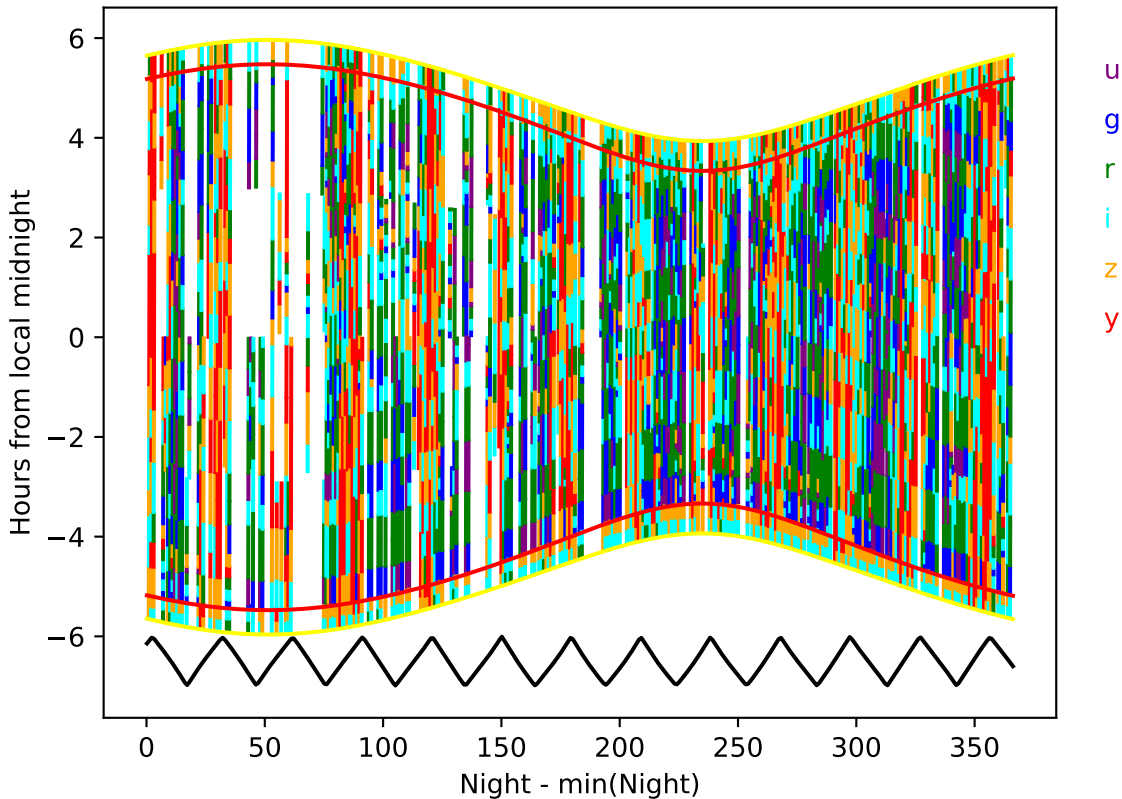
roll_uniform_eh_acc0.8_mjdp0_v3.4_10yrs year 9-10: Hourglass
