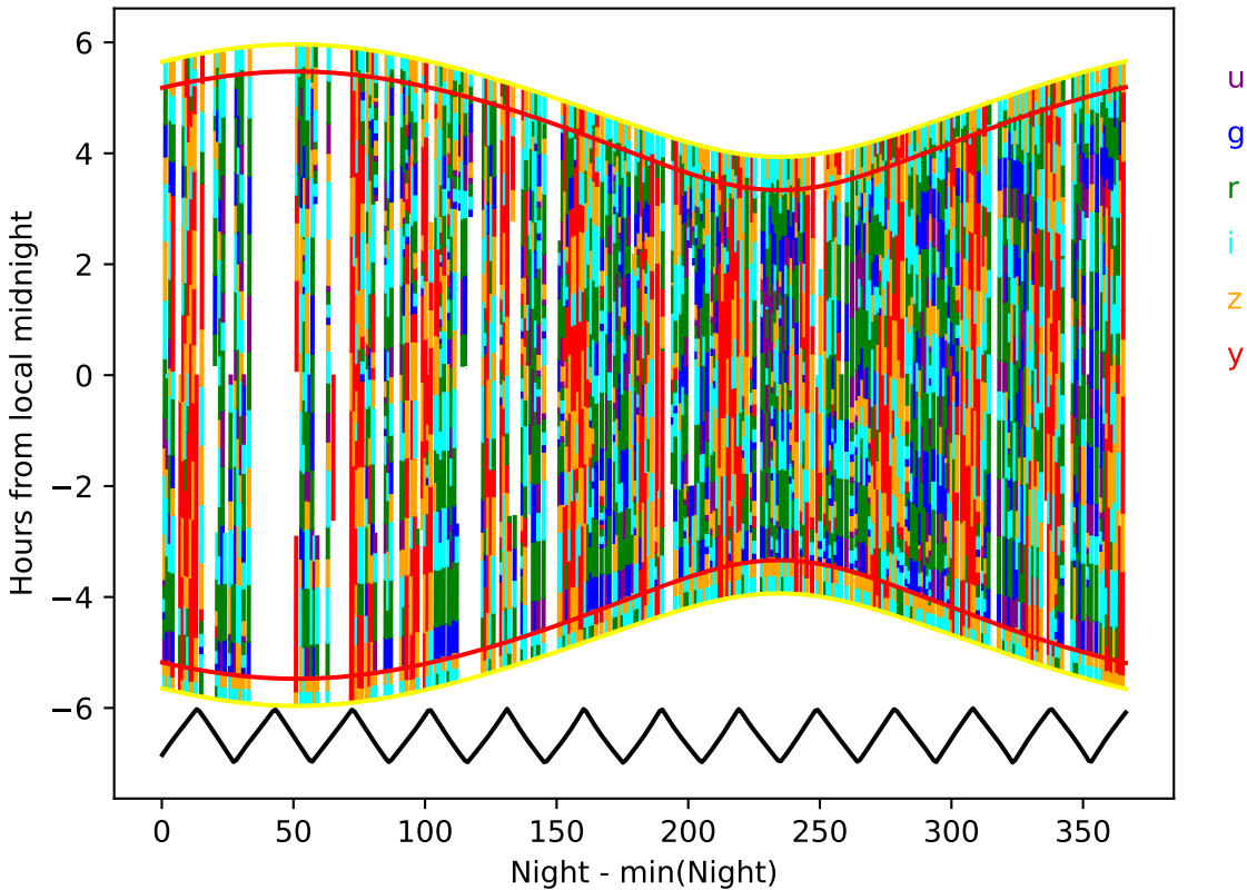
roll_uniform_eh_acc0.8_mjdp0_v3.4_10yrs_year 8-9: Hourglass
