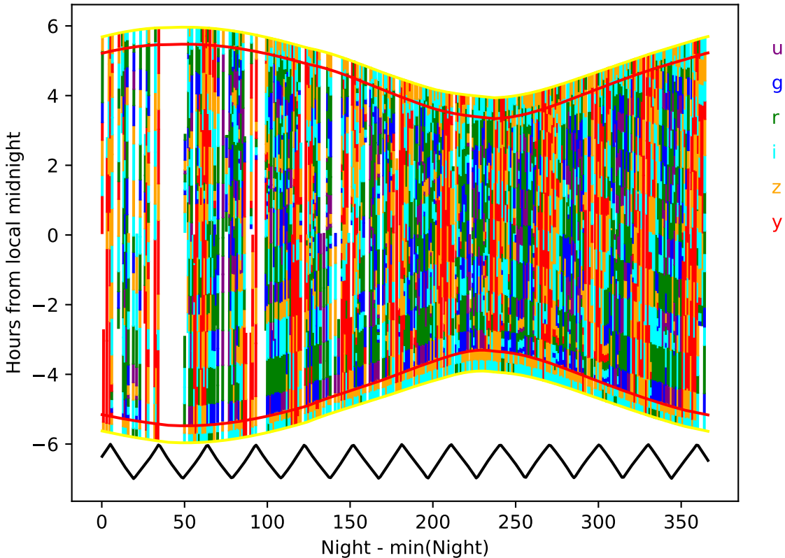
roll_uniform_eh_acc0.8_mjdp0_v3.4_10yrs year 6-7: Hourglass
