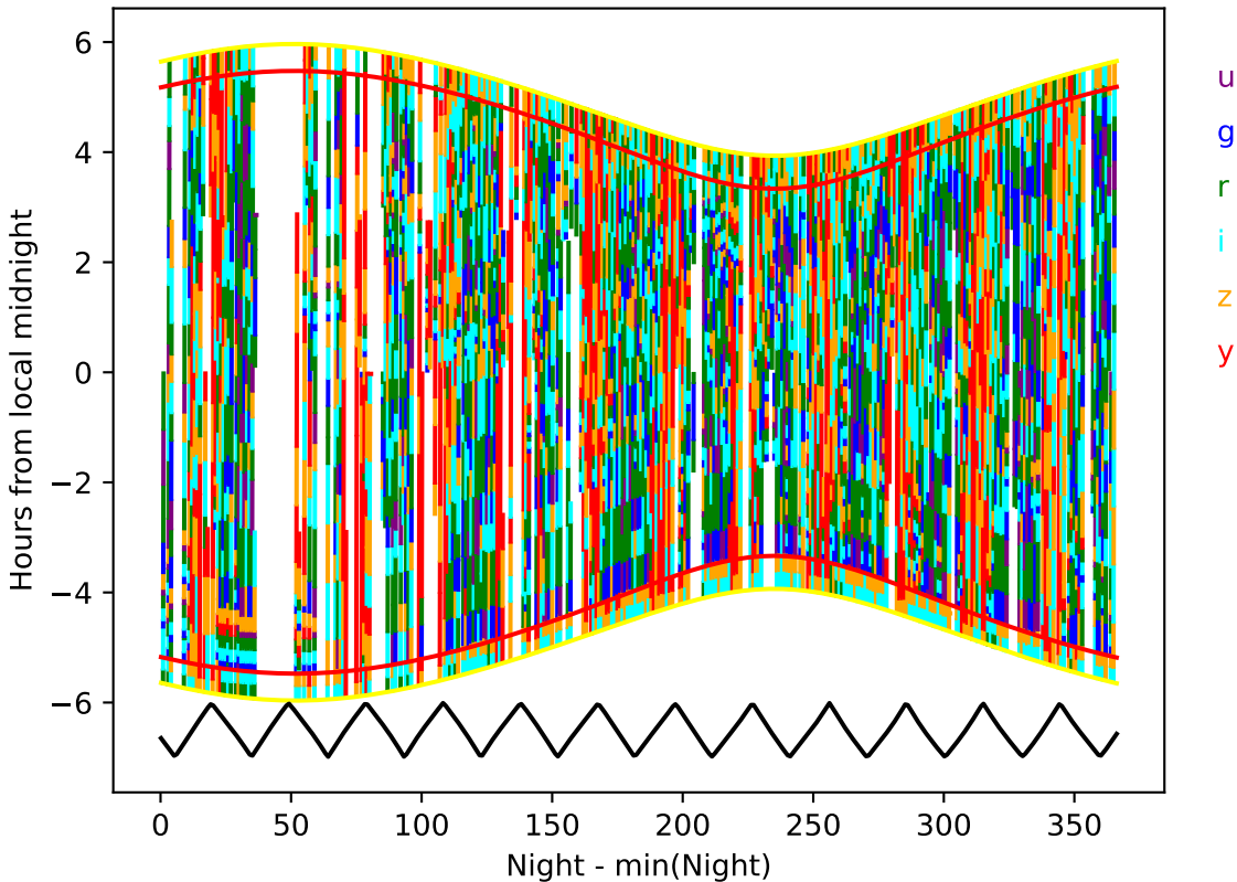
roll_uniform_eh_acc0.8_mjdp0_v3.4_10yrs year 2-3: Hourglass
