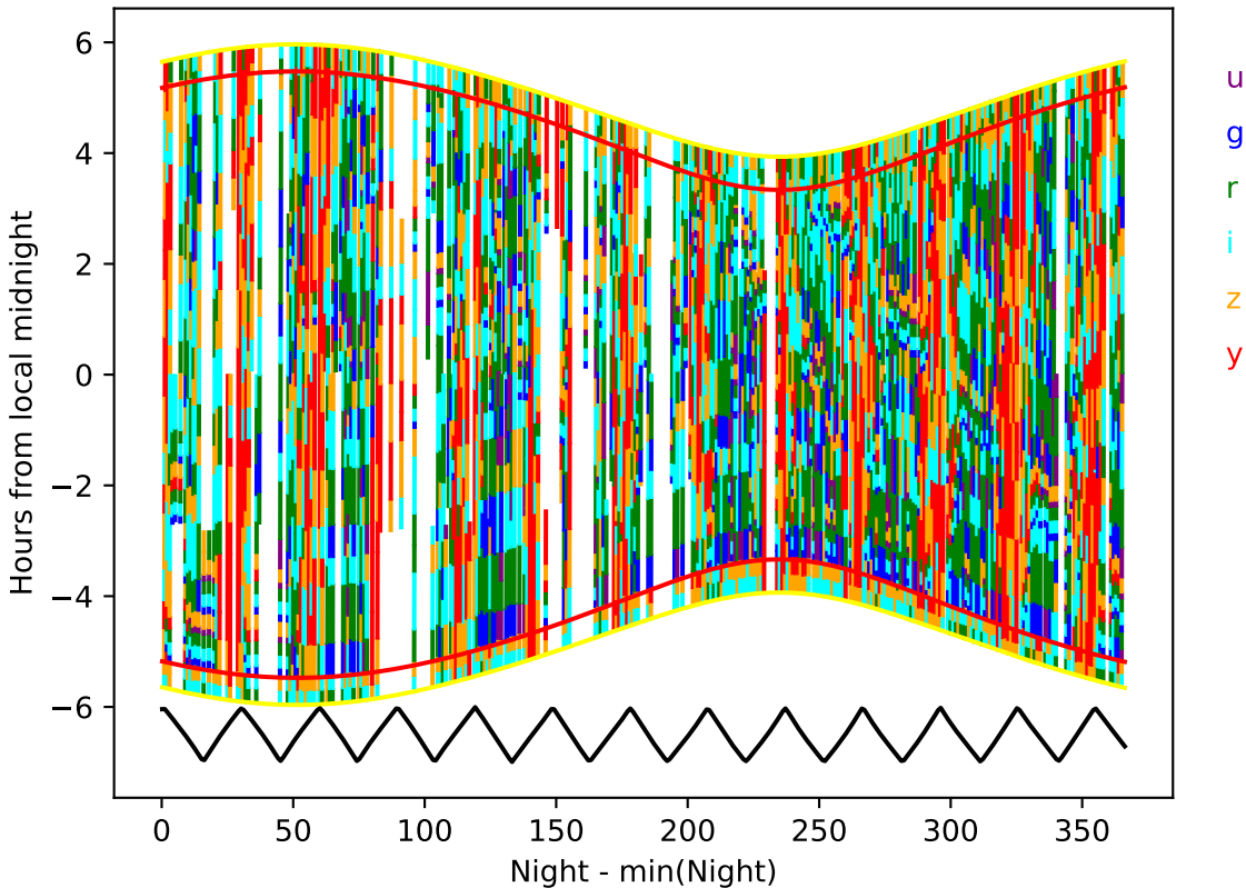
roll_uniform_eh_acc0.8_mjdp0_v3.4_10yrs year 1-2: Hourglass
