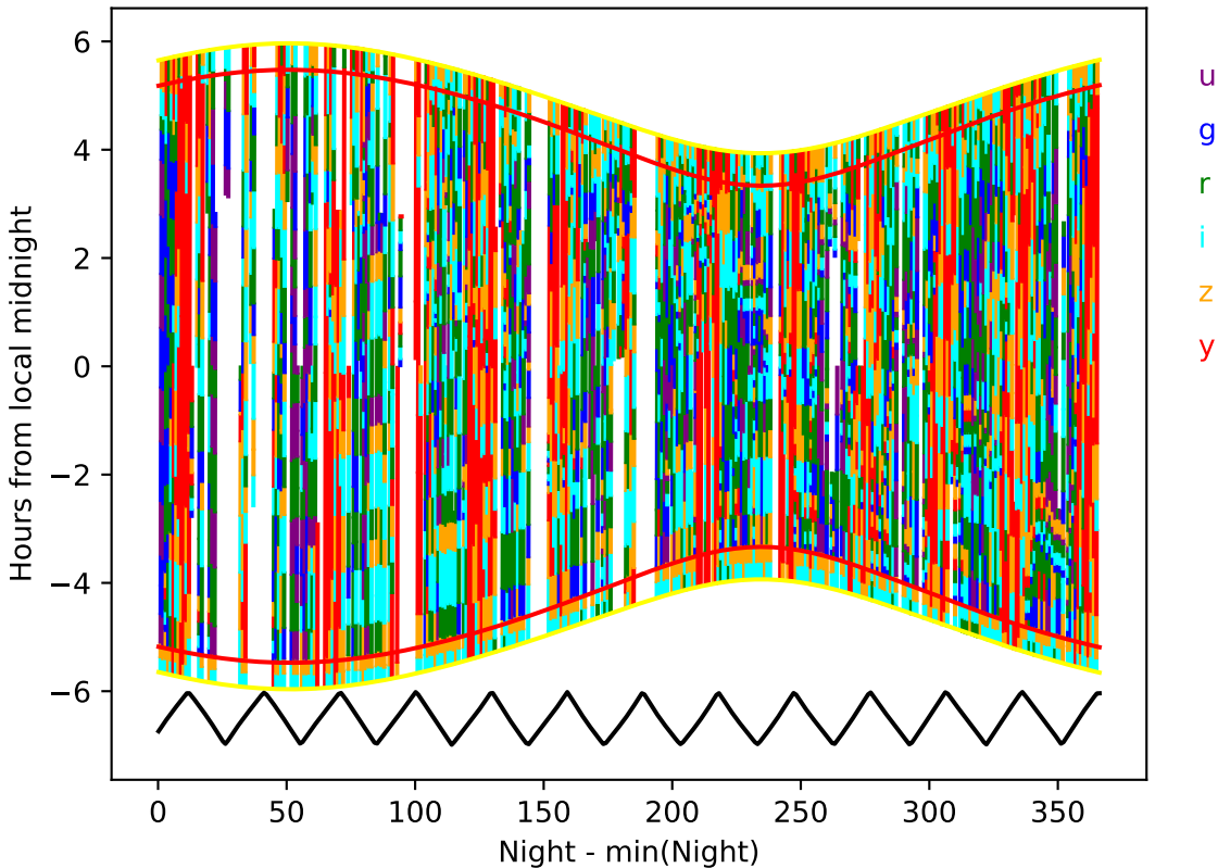
roll_uniform_eh_acc0.8_mjdp0_v3.4_10yrs year 0-1: Hourglass
