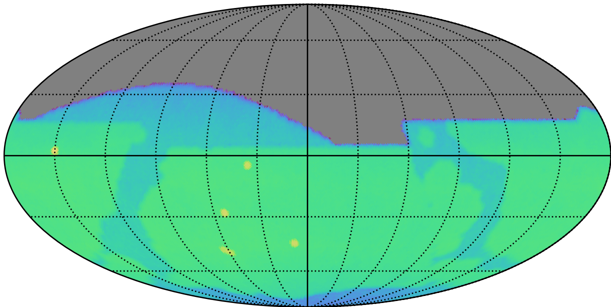
roll_uniform_eh_acc0.8_mjdp0_v3.4_10yrs i: CoaddM5
