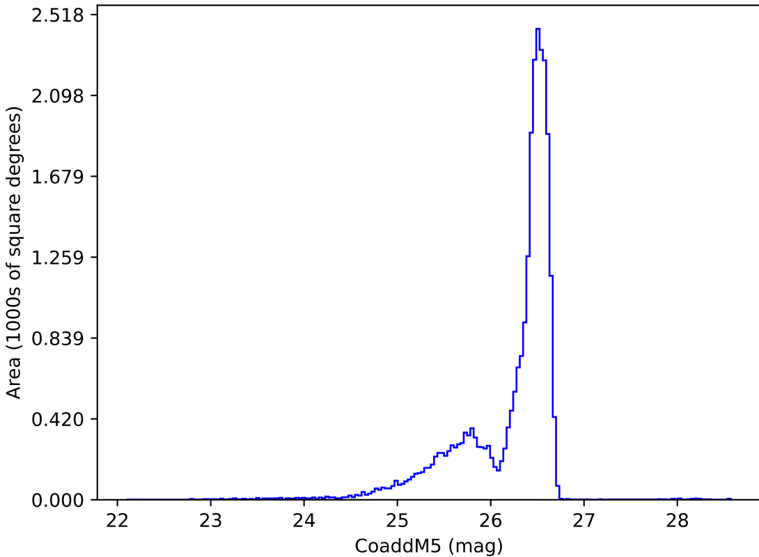
roll_uniform_eh_acc0.8_mjdp0_v3.4_10yrs i: CoaddM5
