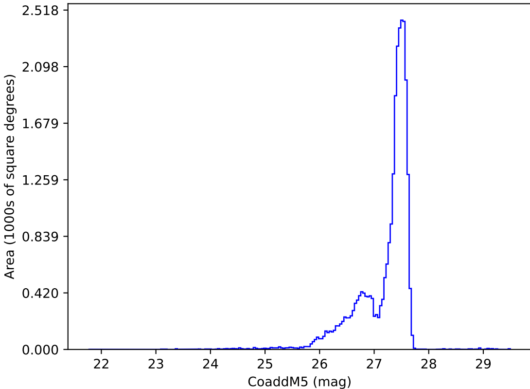
roll_uniform_eh_acc0.8_mjdp0_v3.4_10yrs : CoaddM5
