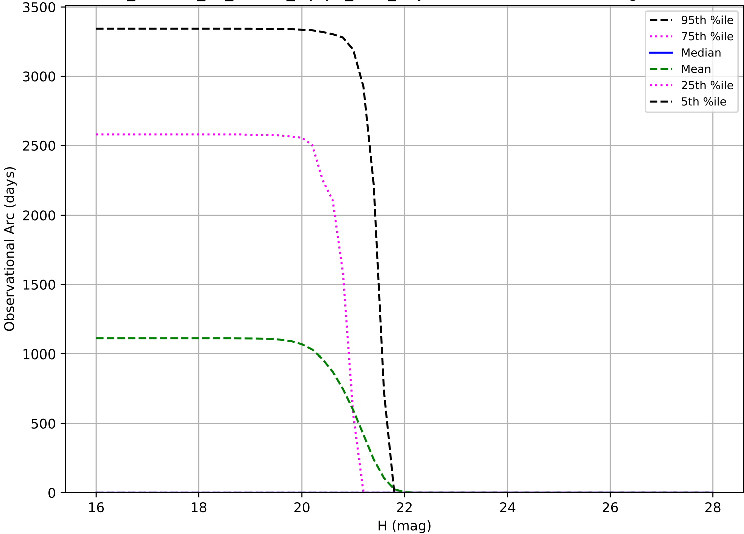
roll_uniform_eh_acc0.5_mjdp0_v3.4_10yrs: Observational Arc Length Vatira
