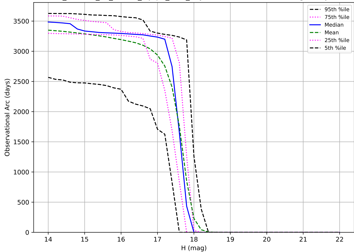
roll_uniform_eh_acc0.5_mjdp0_v3.4_10yrs: Observational Arc Length Trojan
