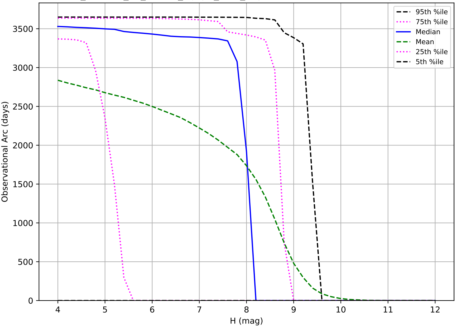
roll_uniform_eh_acc0.5_mjdp0_v3.4_10yrs: Observational Arc Length TNO
