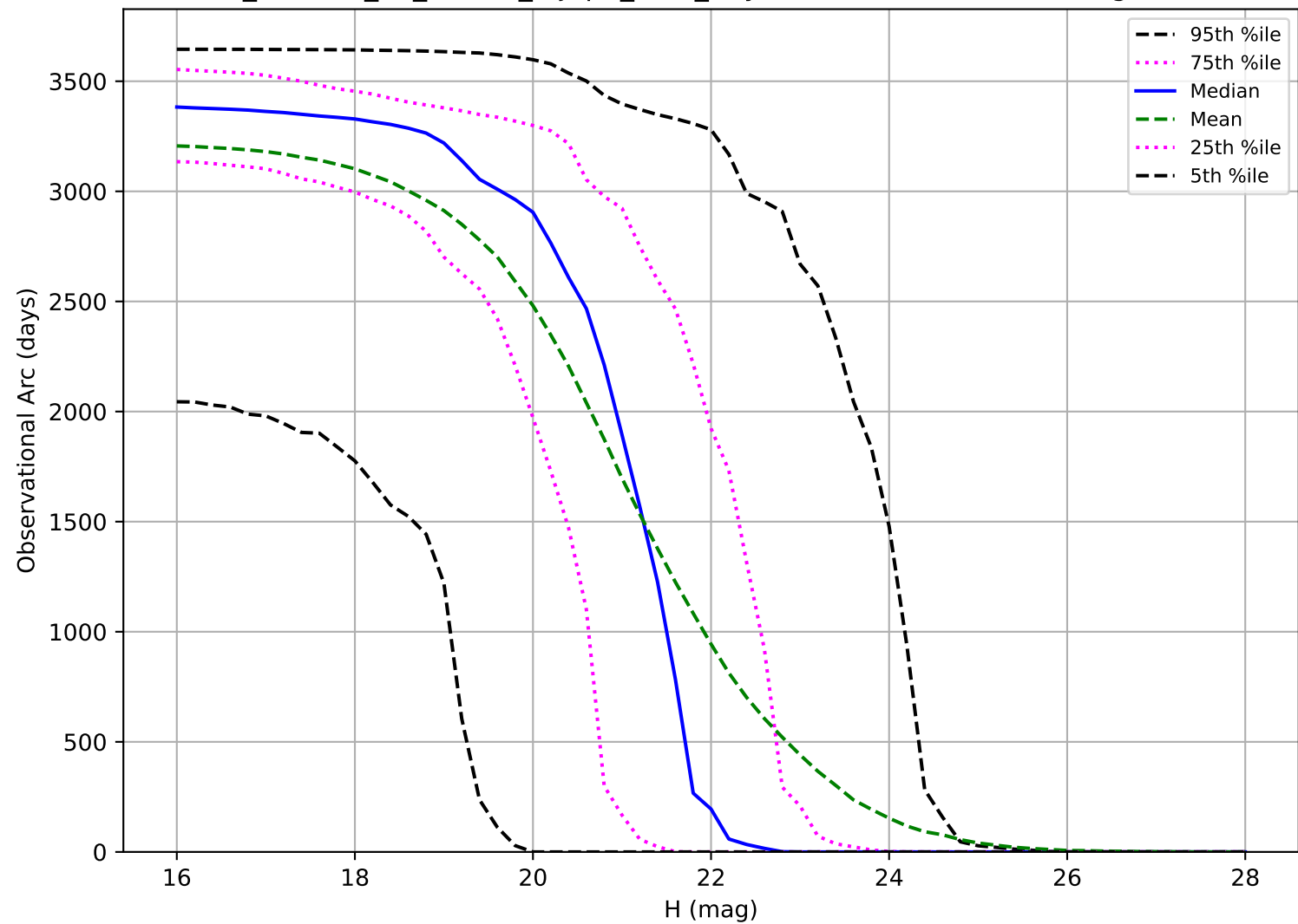
roll_uniform_eh_acc0.5_mjdp0_v3.4_10yrs: Observational Arc Length PHA
