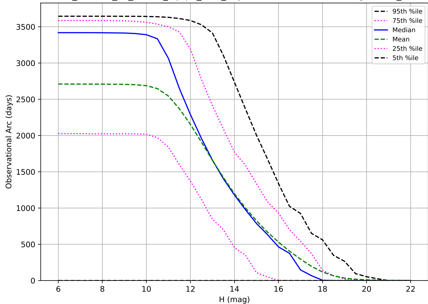
roll_uniform_eh_acc0.5_mjdp0_v3.4_10yrs: Observational Arc Length OCC_r5
