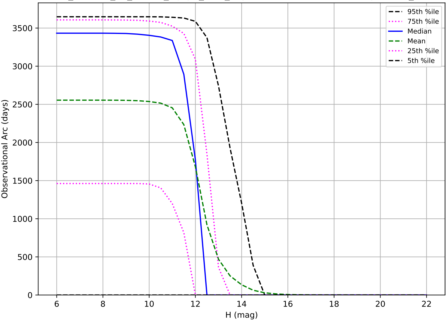
roll_uniform_eh_acc0.5_mjdp0_v3.4_10yrs: Observational Arc Length OCC_r20
