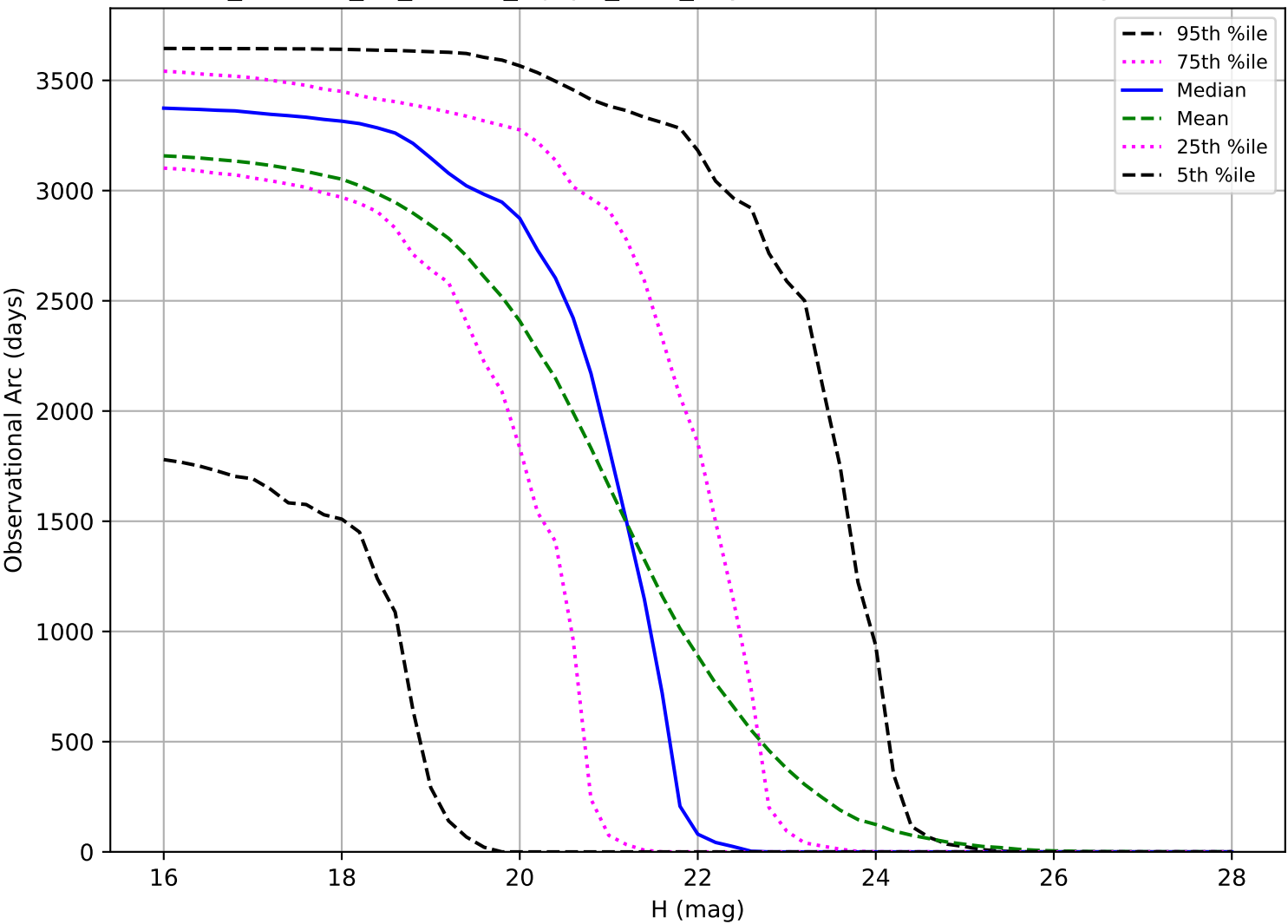
roll_uniform_eh_acc0.5_mjdp0_v3.4_10yrs: Observational Arc Length NEO
