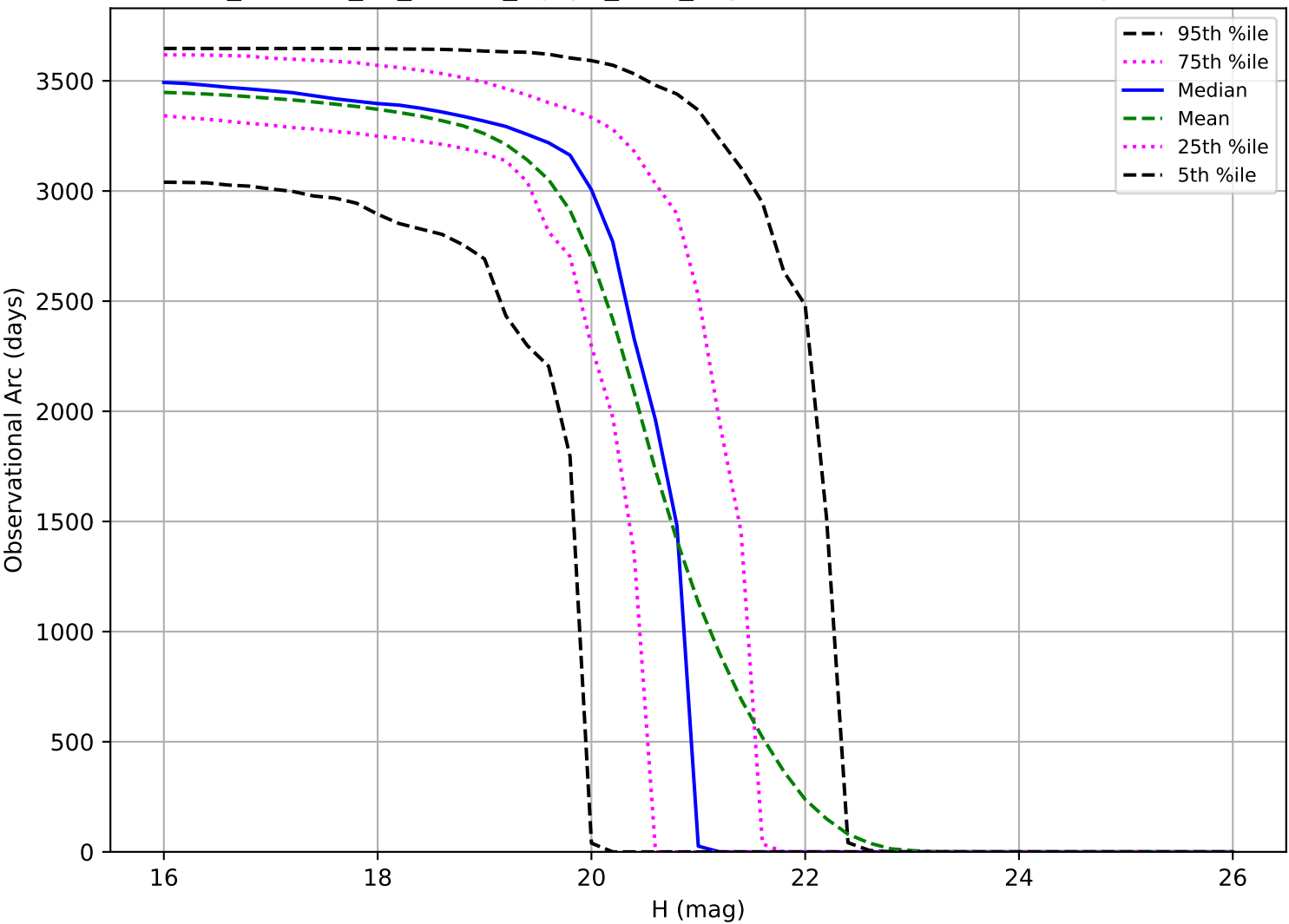
roll_uniform_eh_acc0.5_mjdp0_v3.4_10yrs: Observational Arc Length MBA
