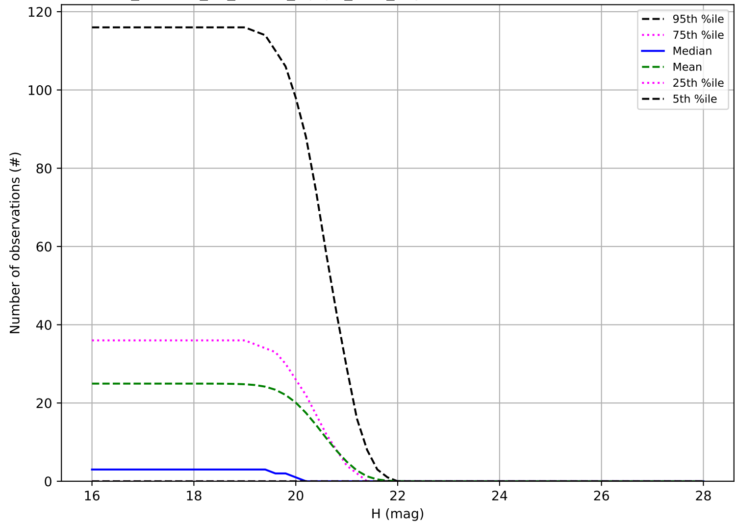
roll_uniform_eh_acc0.5_mjdp0_v3.4_10yrs: Number of observations Vatira
