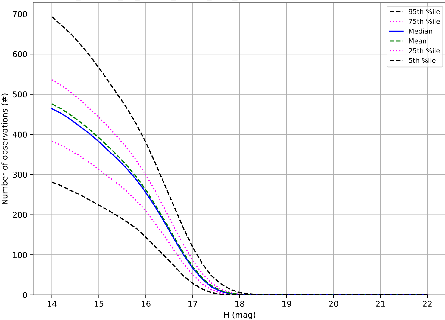
roll_uniform_eh_acc0.5_mjdp0_v3.4_10yrs: Number of observations Trojan
