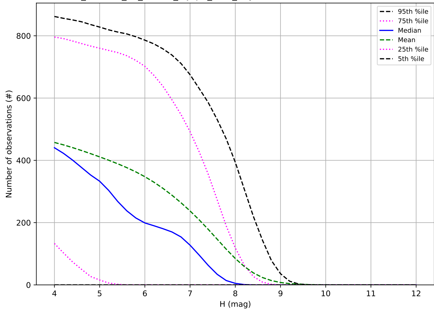
roll_uniform_eh_acc0.5_mjdp0_v3.4_10yrs: Number of observations TNO
