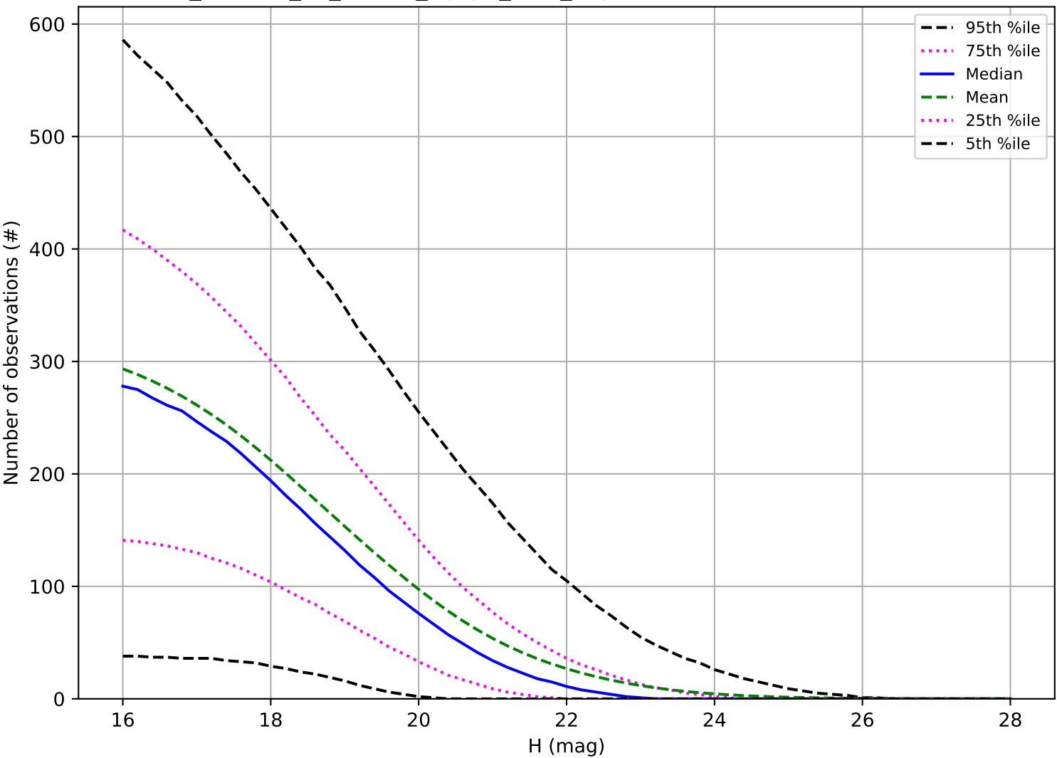
roll_uniform_eh_acc0.5_mjdp0_v3.4_10yrs: Number of observations PHA
