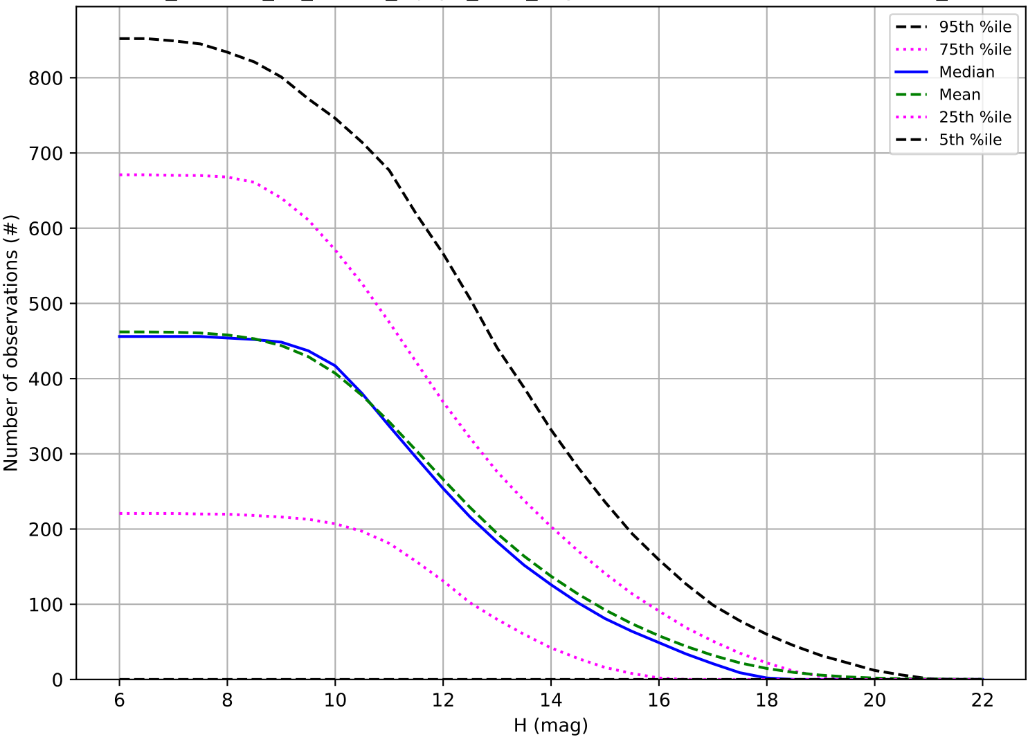
roll_uniform_eh_acc0.5_mjdp0_v3.4_10yrs: Number of observations OCC_r5
