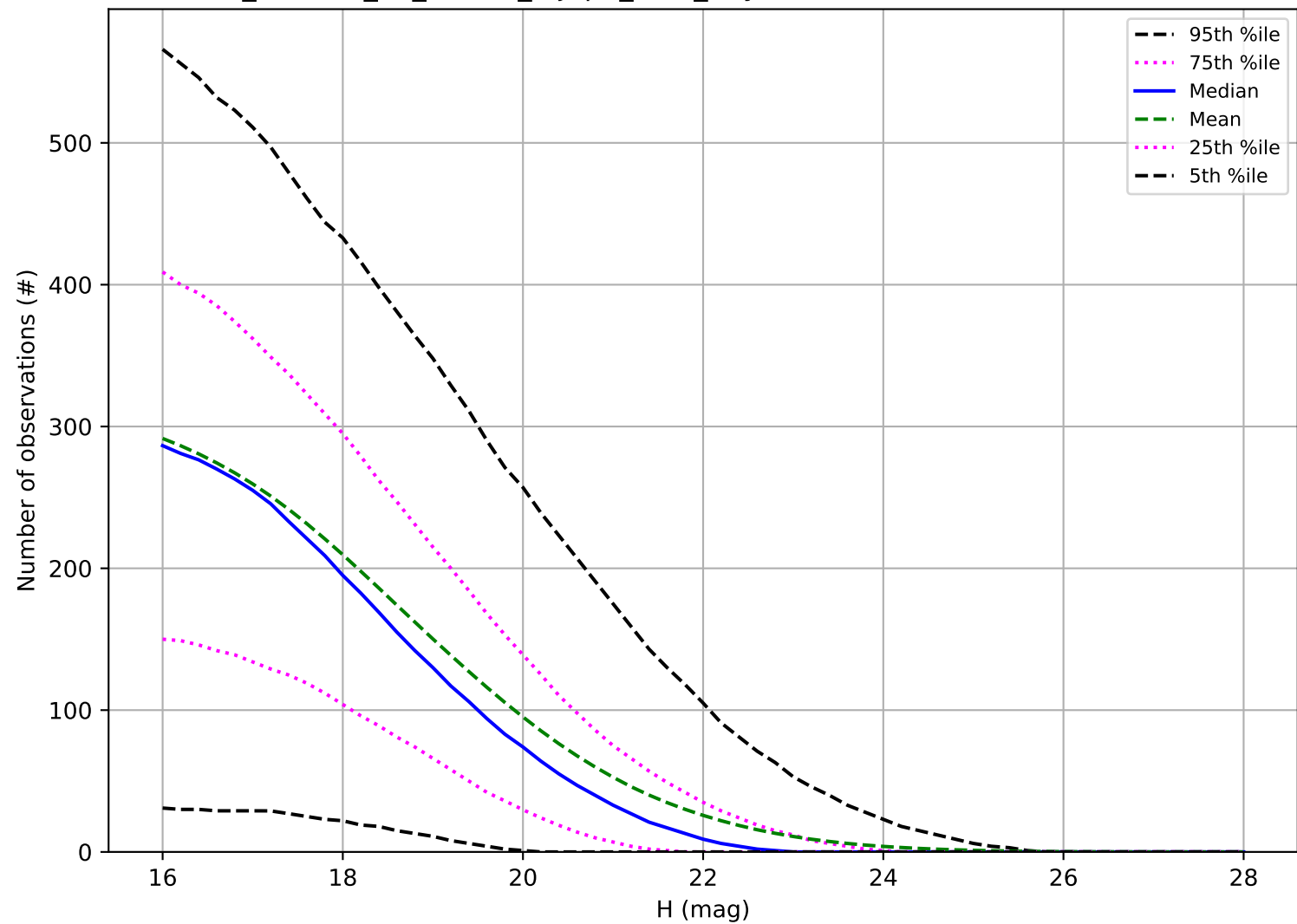
roll_uniform_eh_acc0.5_mjdp0_v3.4_10yrs: Number of observations NEO
