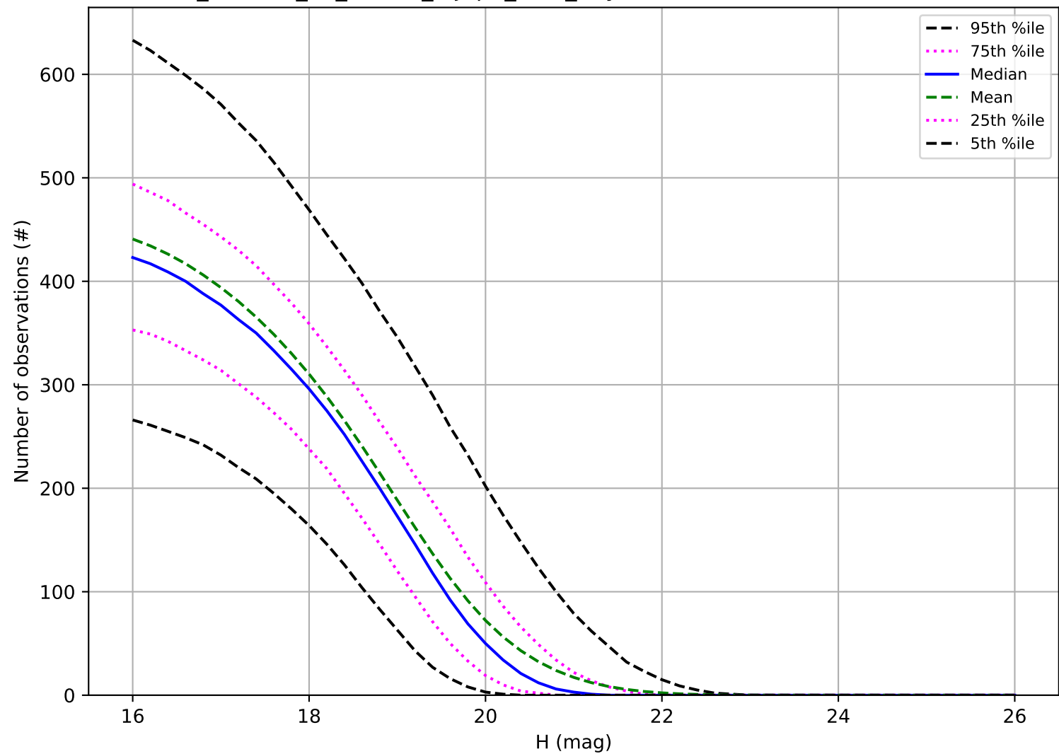
roll_uniform_eh_acc0.5_mjdp0_v3.4_10yrs: Number of observations MBA
