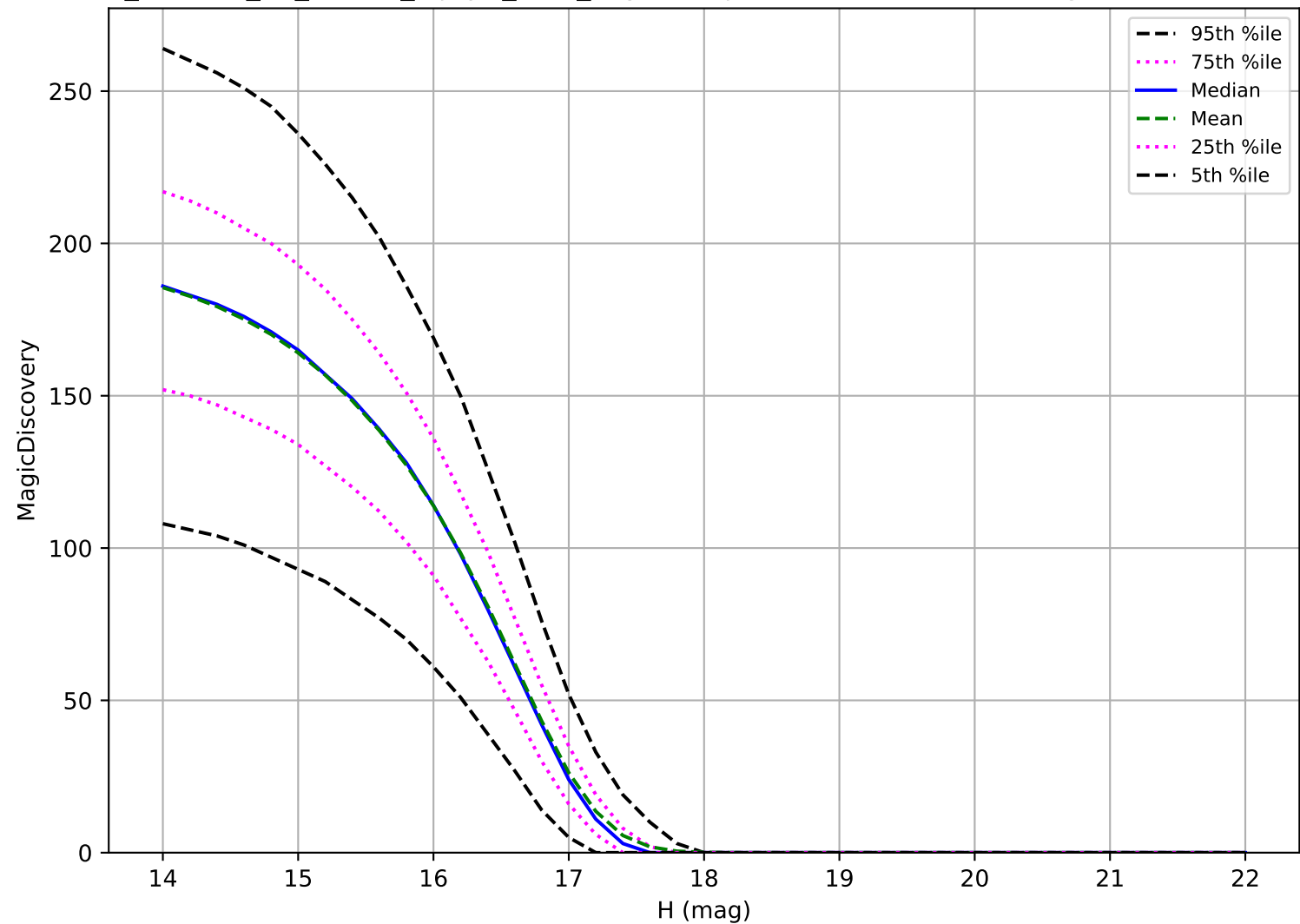
roll_uniform_eh_acc0.5_mjdp0_v3.4_10yrs: Trojan 6 detections in 60 nights detection loss
