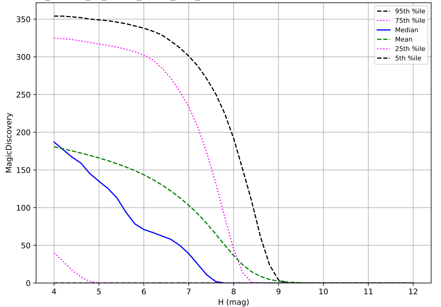
roll_uniform_eh_acc0.5_mjdp0_v3.4_10yrs: TNO 6 detections in 60 nights detection loss
