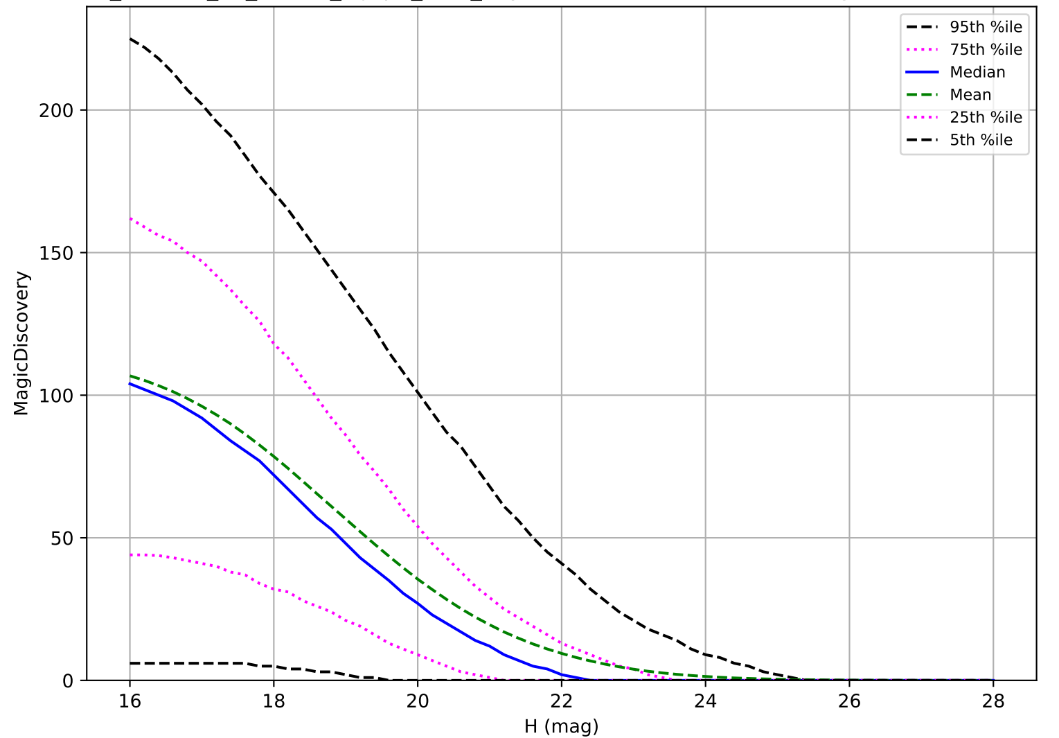
roll_uniform_eh_acc0.5_mjdp0_v3.4_10yrs: PHA 6 detections in 60 nights detection loss
