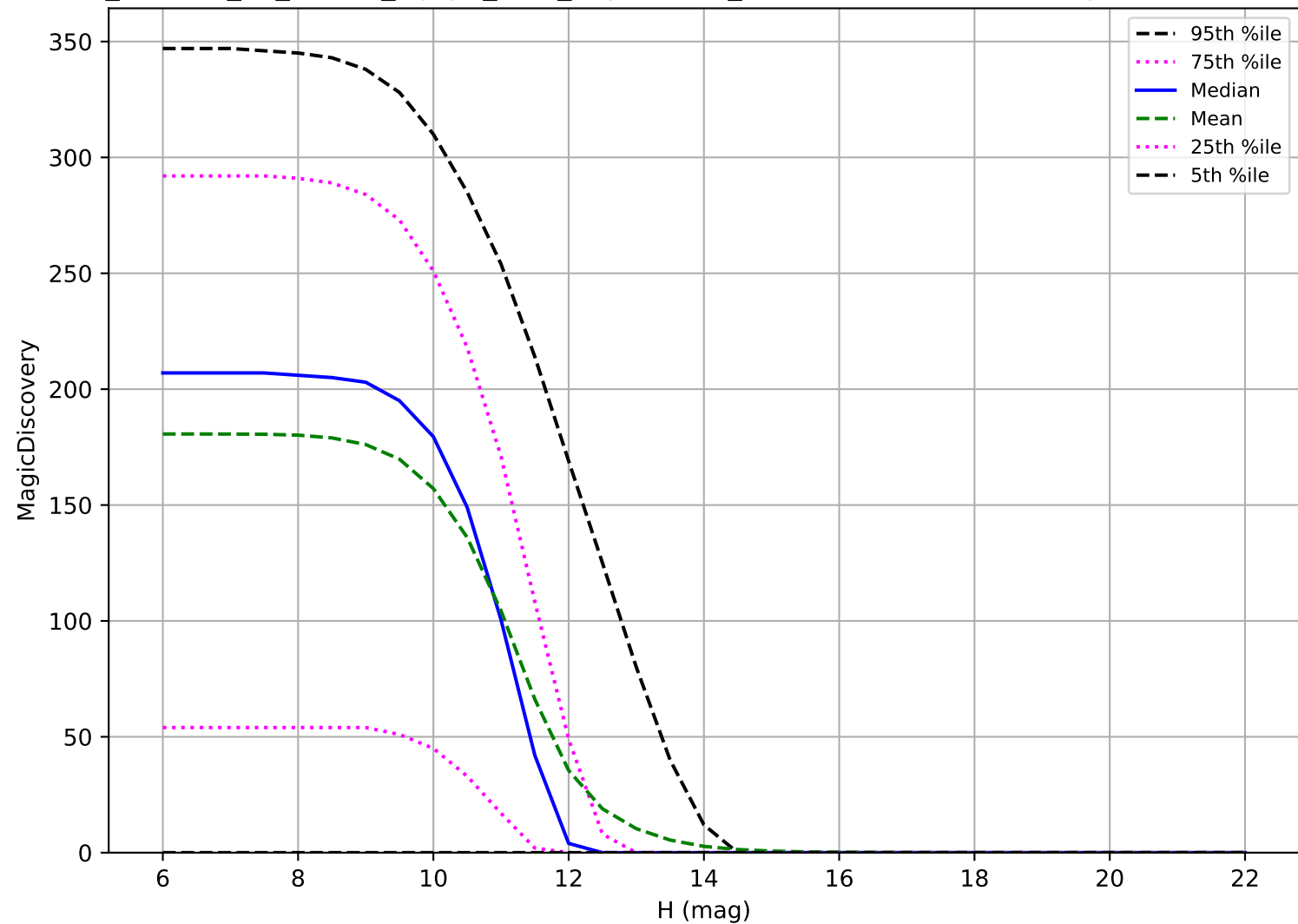
roll_uniform_eh_acc0.5_mjdp0_v3.4_10yrs: OCC_r20 6 detections in 60 nights detection loss
