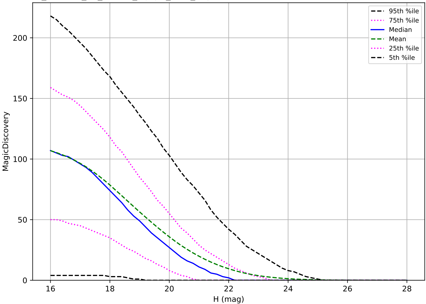
roll_uniform_eh_acc0.5_mjdp0_v3.4_10yrs: NEO 6 detections in 60 nights detection loss
