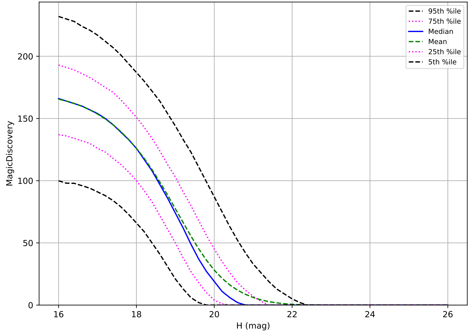
roll_uniform_eh_acc0.5_mjdp0_v3.4_10yrs: MBA 6 detections in 60 nights detection loss
