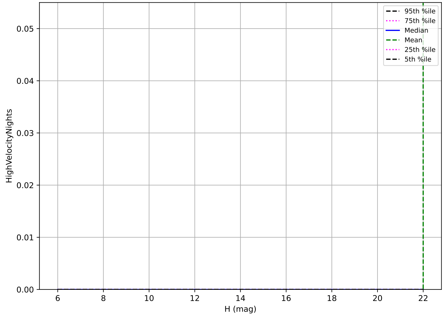
roll_uniform_eh_acc0.5_mjdp0_v3.4_10yrs: OCC_r20 High velocity pair detection loss
