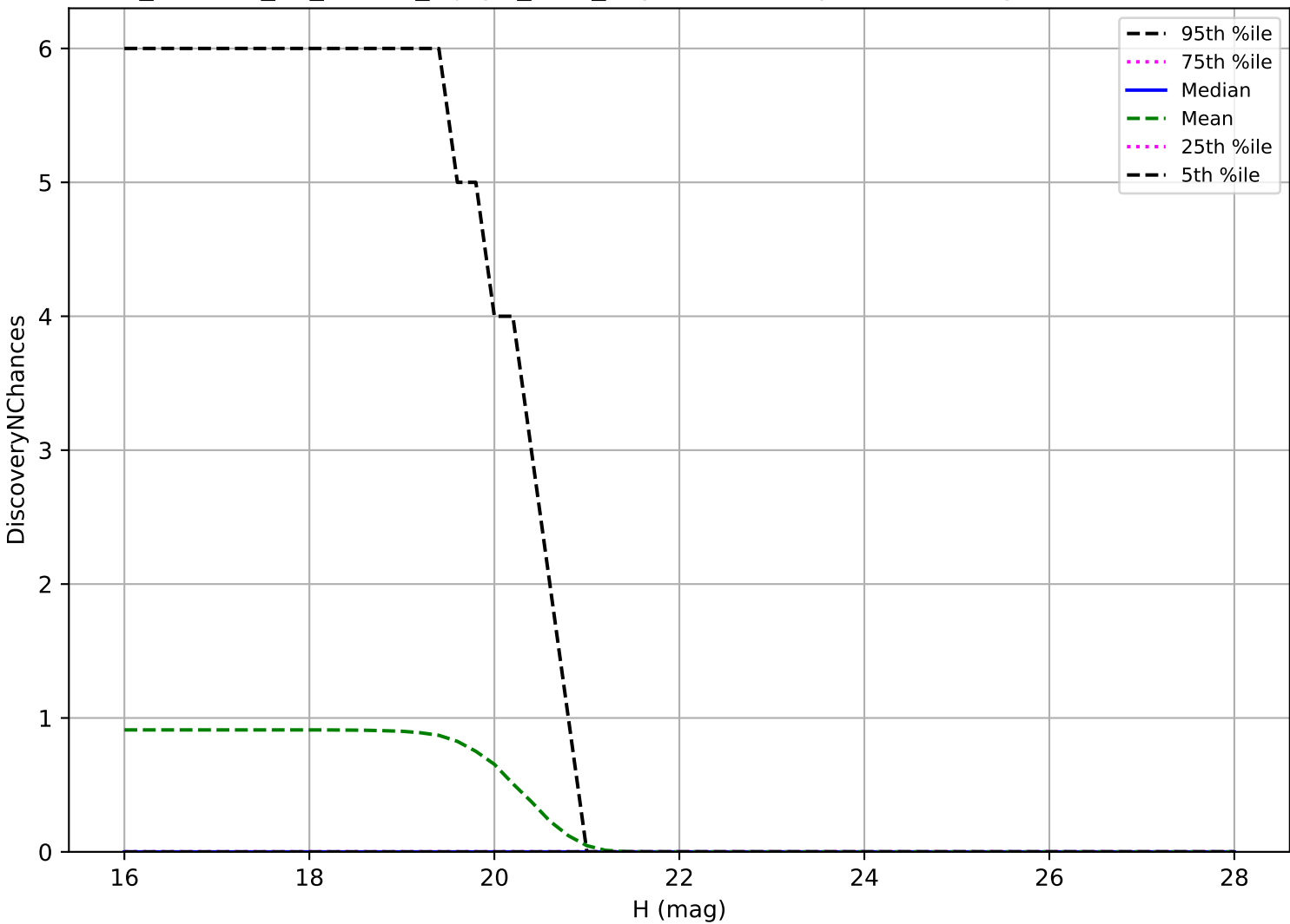
roll_uniform_eh_acc0.5_mjdp0_v3.4_10yrs: Vatira 3 pairs in 15 nights detection loss
