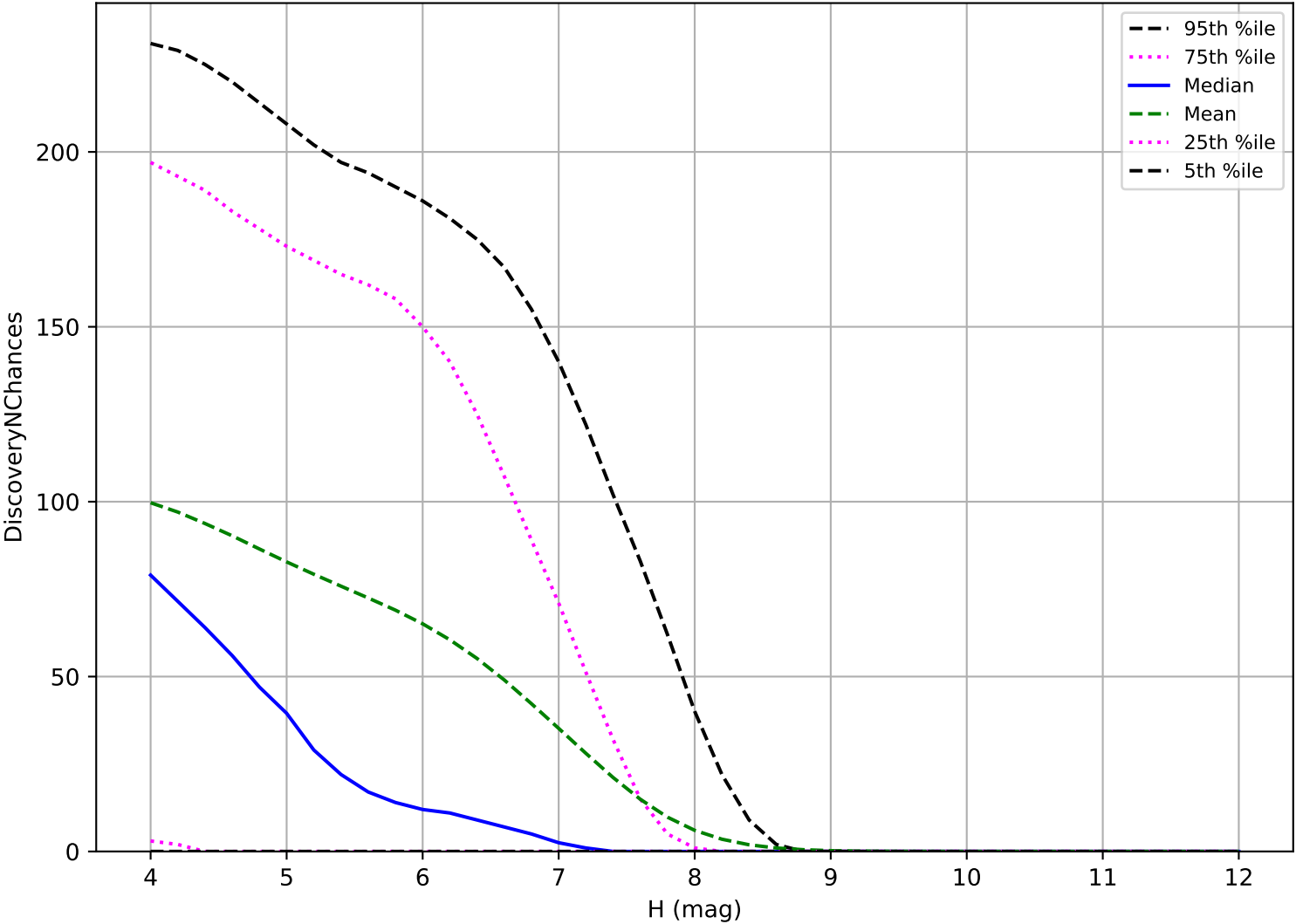
roll_uniform_eh_acc0.5_mjdp0_v3.4_10yrs: TNO 3 pairs in 15 nights detection loss
