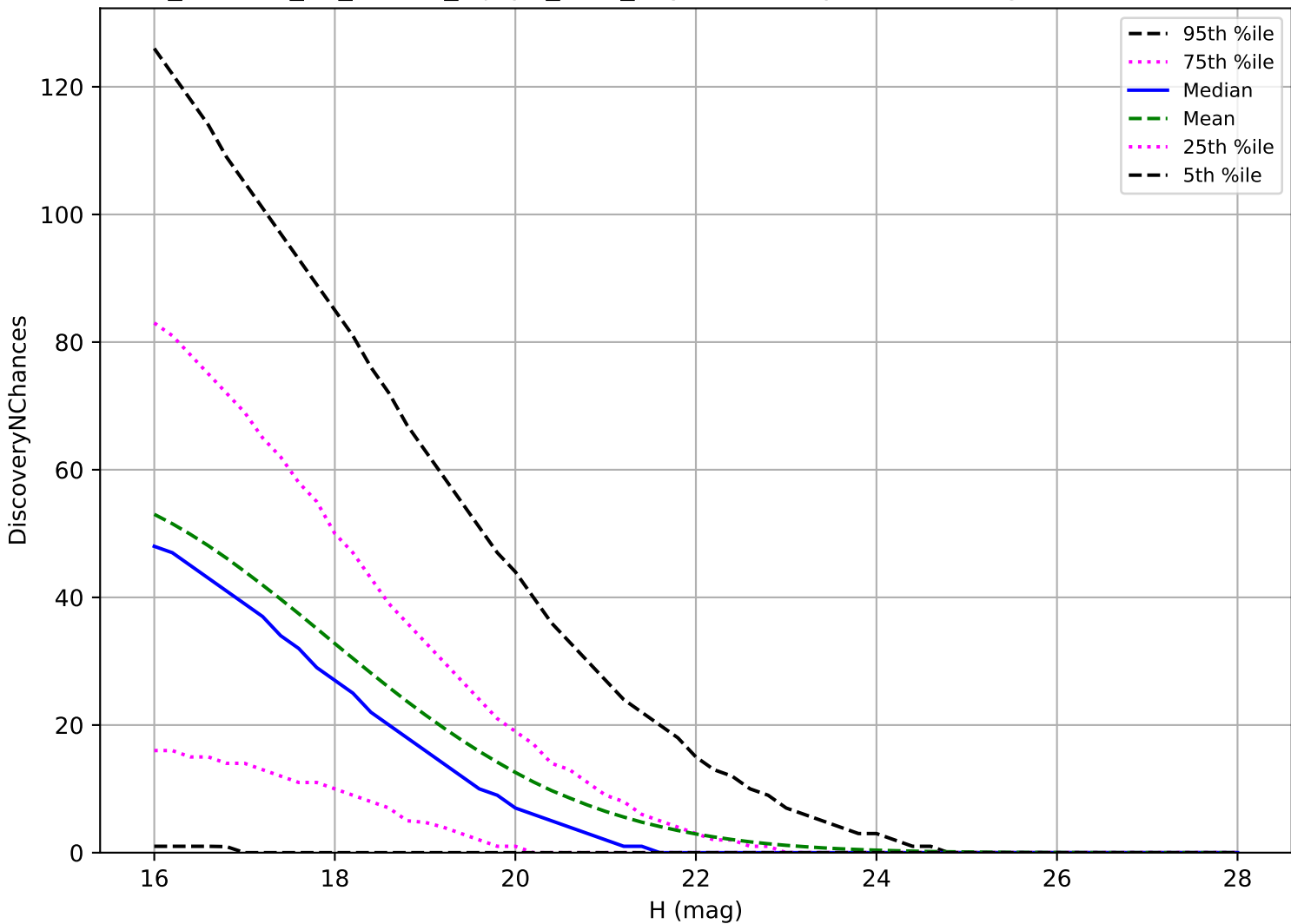
roll_uniform_eh_acc0.5_mjdp0_v3.4_10yrs: PHA 3 pairs in 15 nights detection loss
