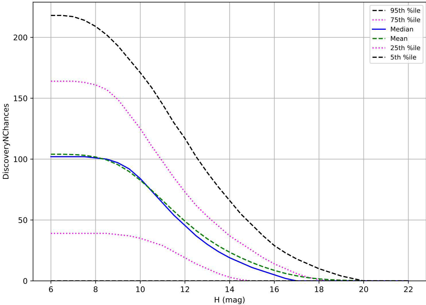
roll_uniform_eh_acc0.5_mjdp0_v3.4_10yrs: OCC_r5 3 pairs in 15 nights detection loss
