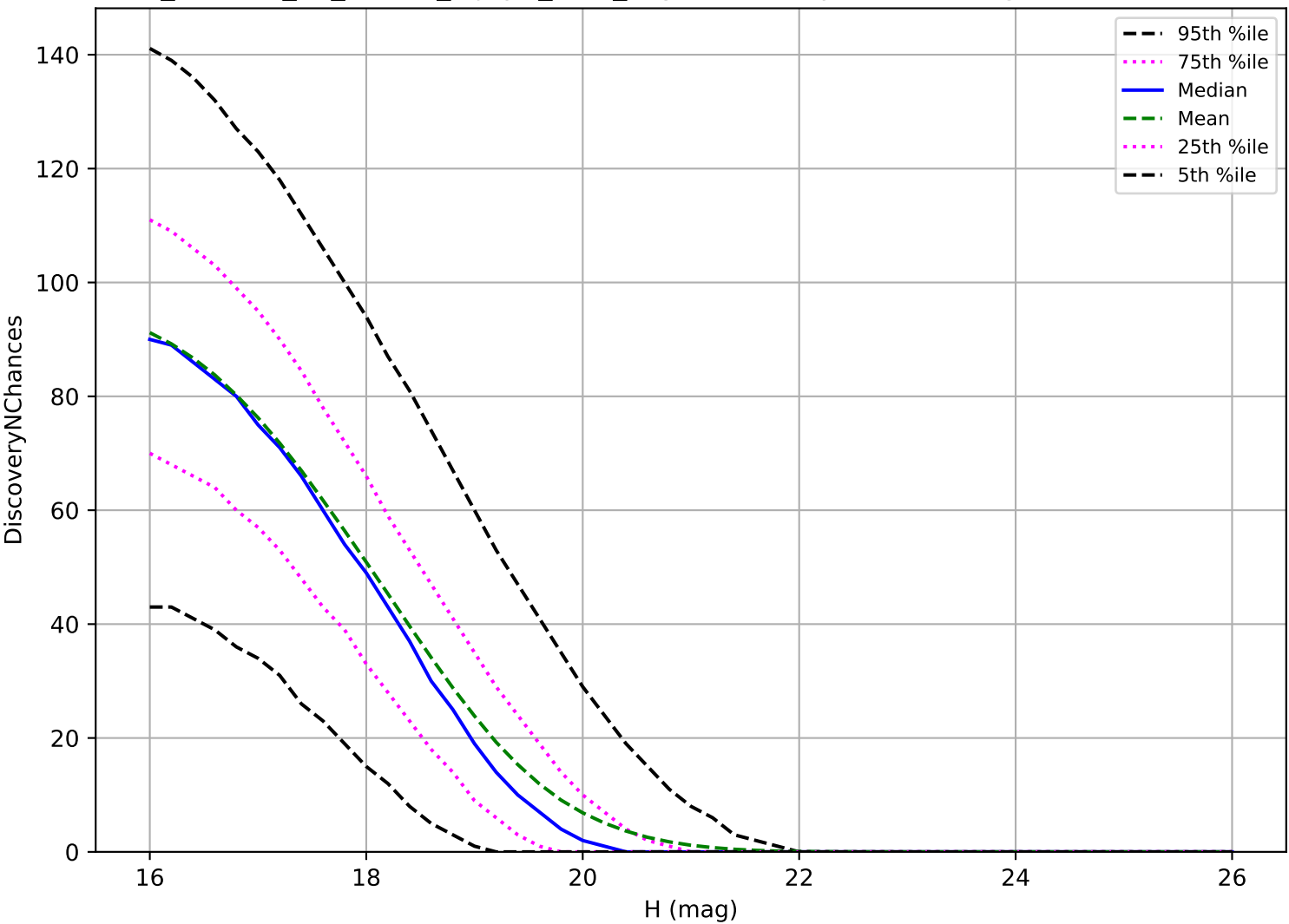
roll_uniform_eh_acc0.5_mjdp0_v3.4_10yrs: MBA 3 pairs in 15 nights detection loss
