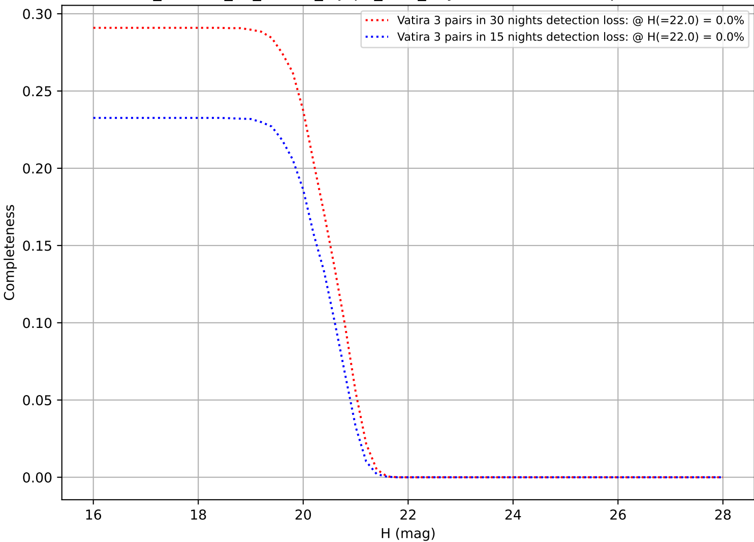
roll_uniform_eh_acc0.5_mjdp0_v3.4_10yrs: DifferentialCompleteness
