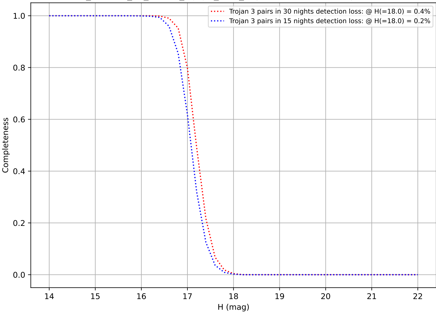
roll_uniform_eh_acc0.5_mjdp0_v3.4_10yrs: DifferentialCompleteness
