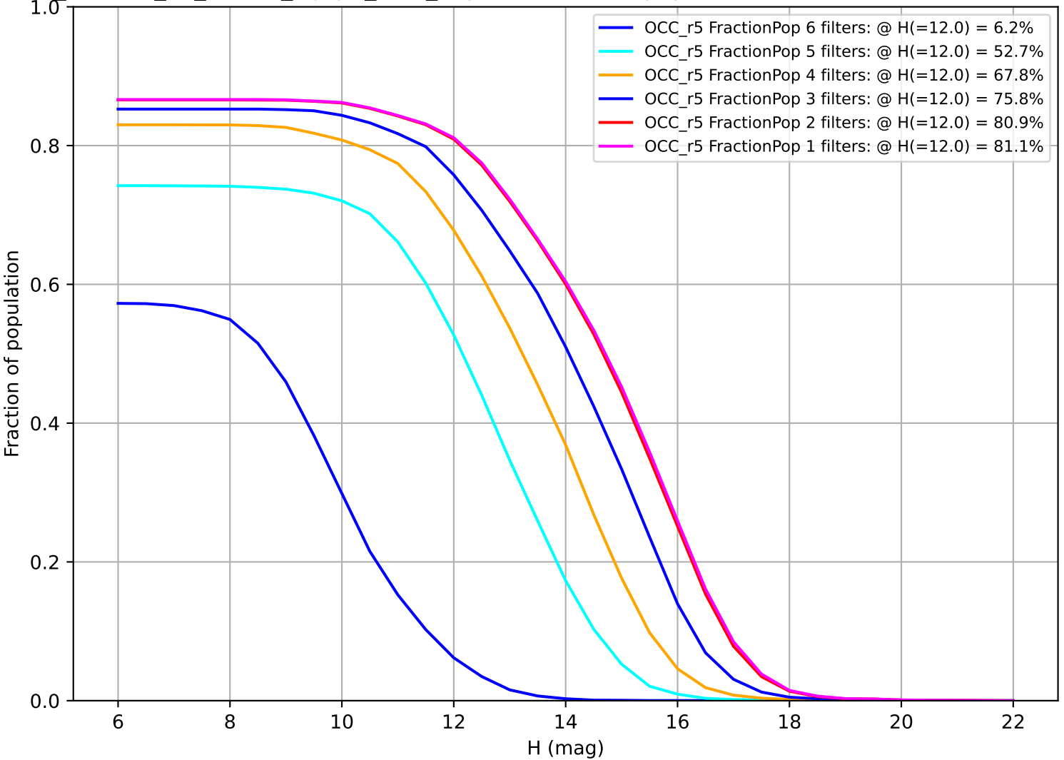
roll_uniform_eh_acc0.5_mjdp0_v3.4_10yrs: Fraction of population with colors in X filters OCC_r5
