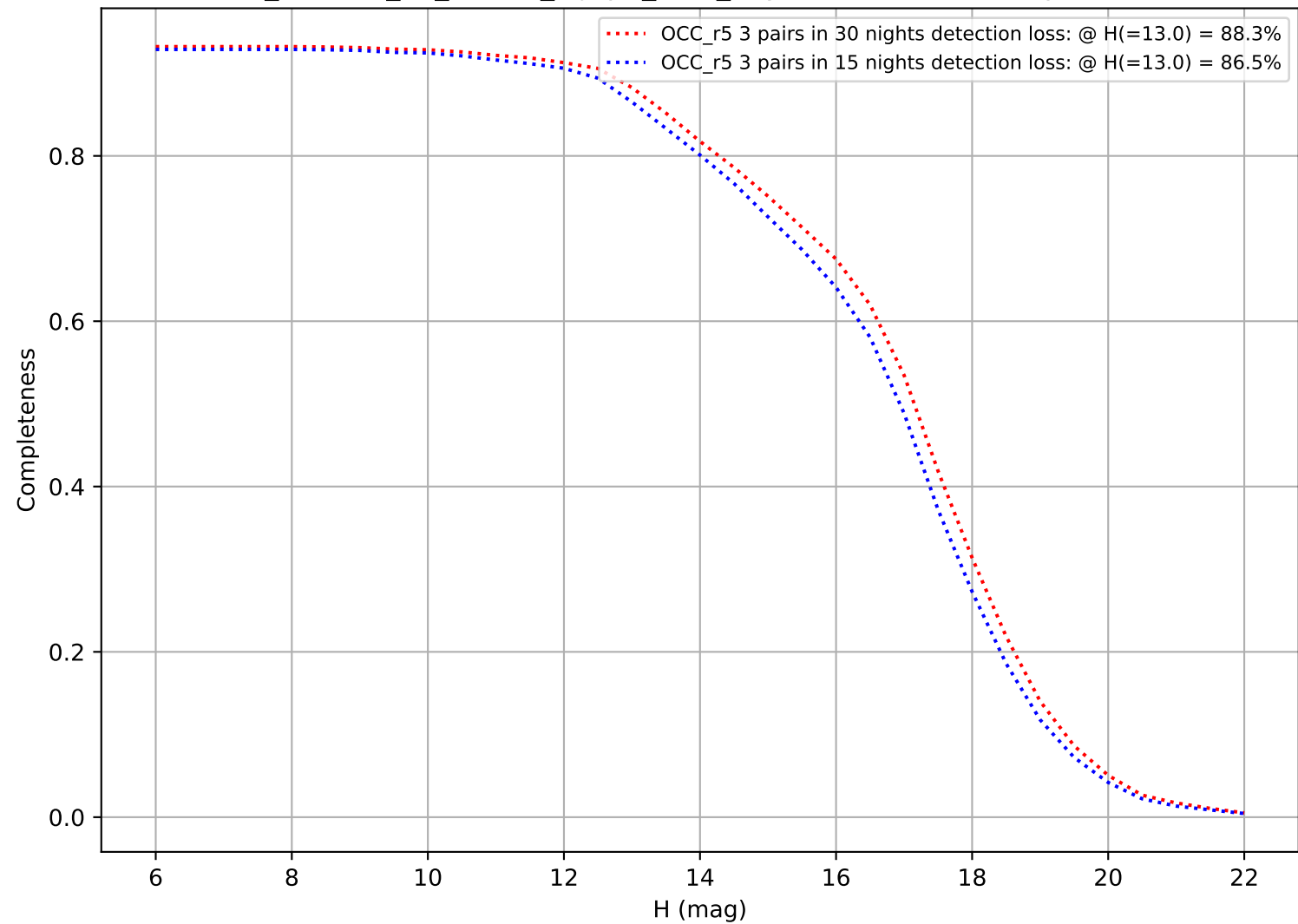
roll_uniform_eh_acc0.5_mjdp0_v3.4_10yrs: DifferentialCompleteness
