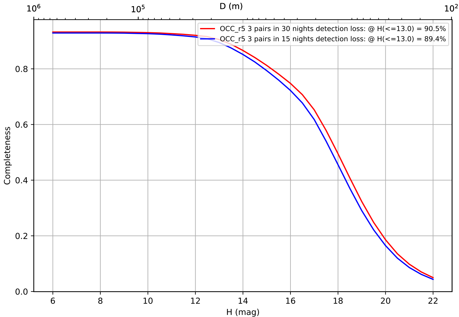
roll_uniform_eh_acc0.5_mjdp0_v3.4_10yrs: CumulativeCompleteness
