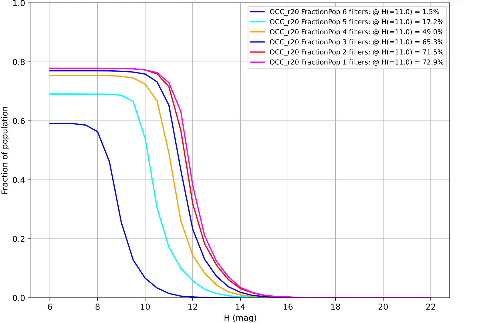
roll_uniform_eh_acc0.5_mjdp0_v3.4_10yrs: Fraction of population with colors in X filters OCC_r20
