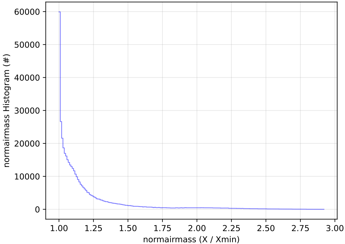
roll_uniform_eh_acc0.5_mjdp0_v3.4_10yrs All sky z band: normairmass Histogram
