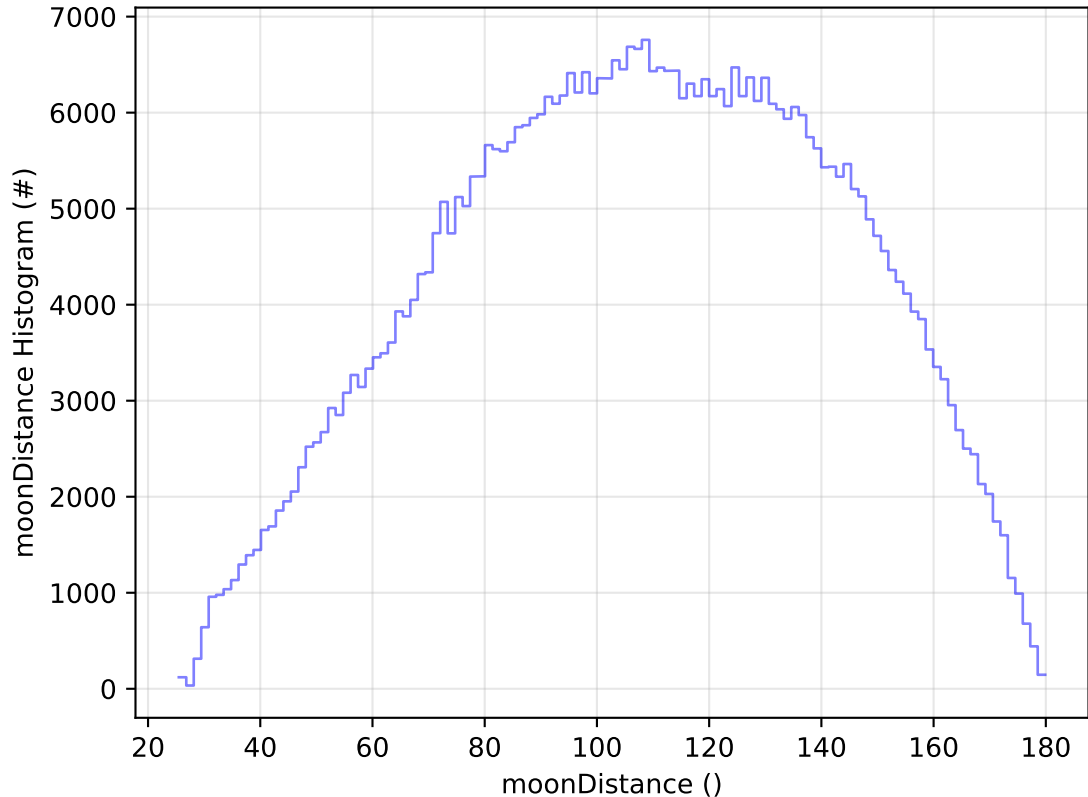
roll_uniform_eh_acc0.5_mjdp0_v3.4_10yrs WFD r band: moonDistance Histogram
