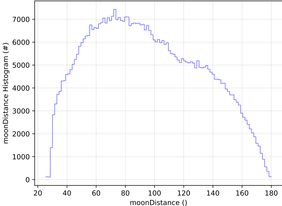
roll_uniform_eh_acc0.5_mjdp0_v3.4_10yrs WFD i band: moonDistance Histogram
