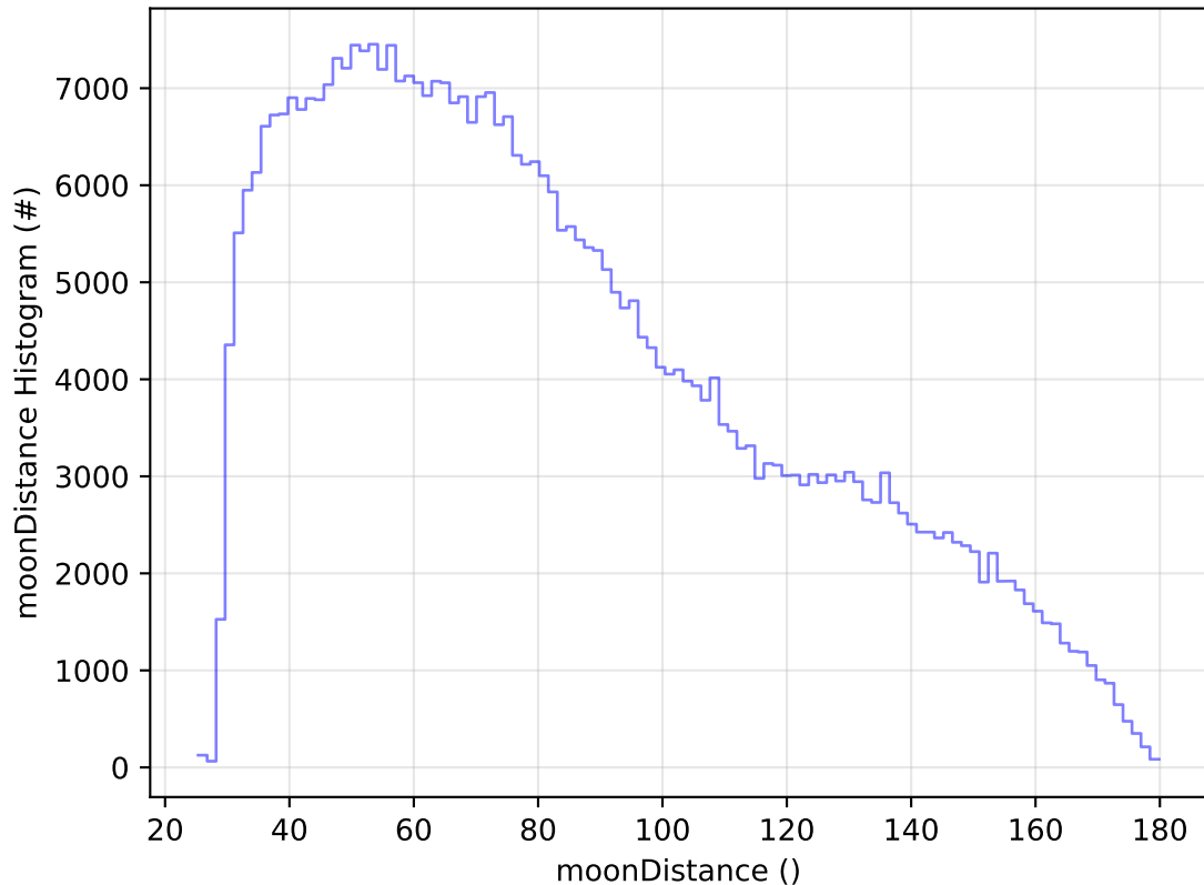
roll_uniform_eh_acc0.5_mjdp0_v3.4_10yrs All sky z band: moonDistance Histogram
