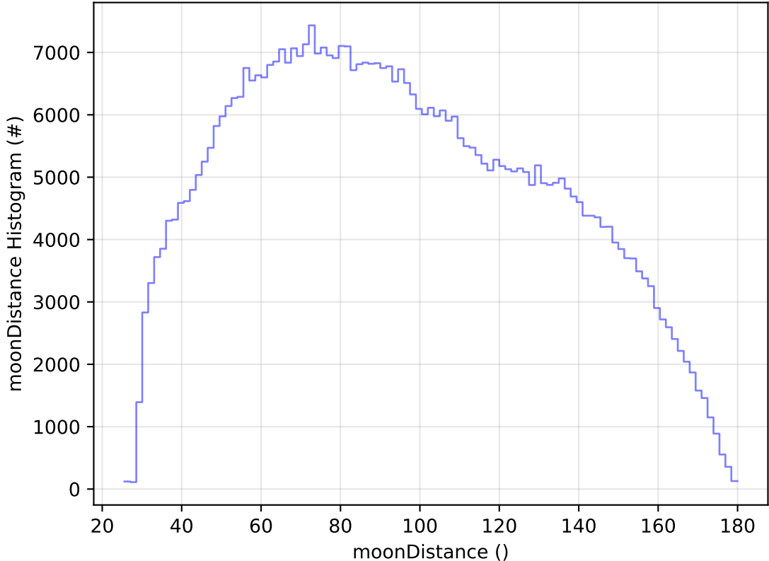
roll_uniform_eh_acc0.5_mjdp0_v3.4_10yrs All sky i band: moonDistance Histogram
