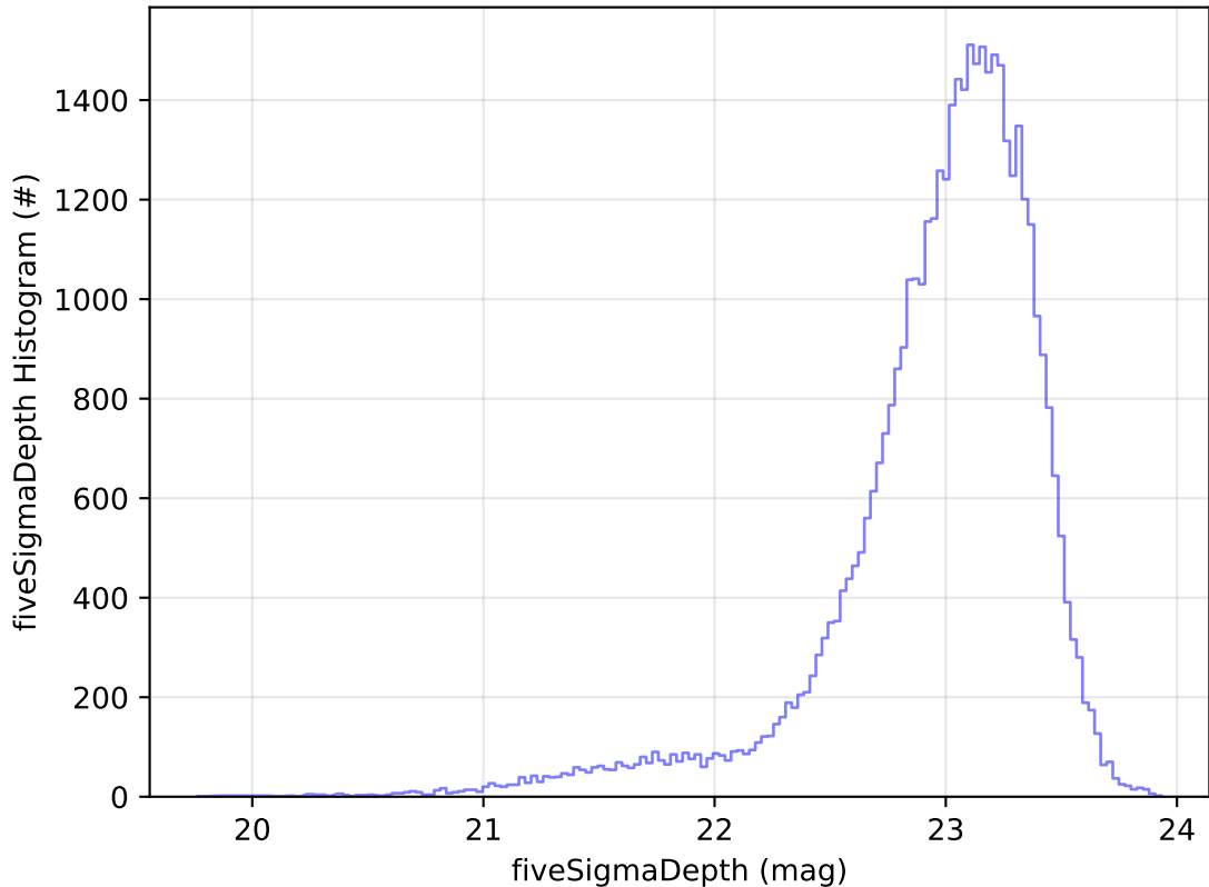
roll_uniform_eh_acc0.5_mjdp0_v3.4_10yrs Yr 1 z band: fiveSigmaDepth Histogram
