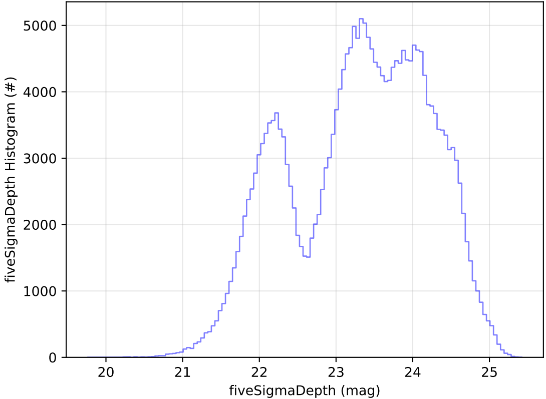
roll_uniform_eh_acc0.5_mjdp0_v3.4_10yrs Yr 1 all bands: fiveSigmaDepth Histogram
