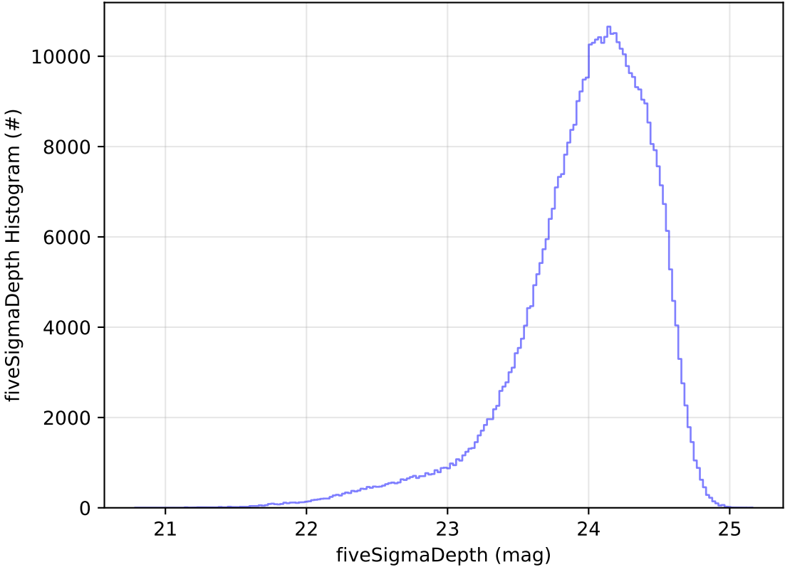
roll_uniform_eh_acc0.5_mjdp0_v3.4_10yrs WFD r band: fiveSigmaDepth Histogram
